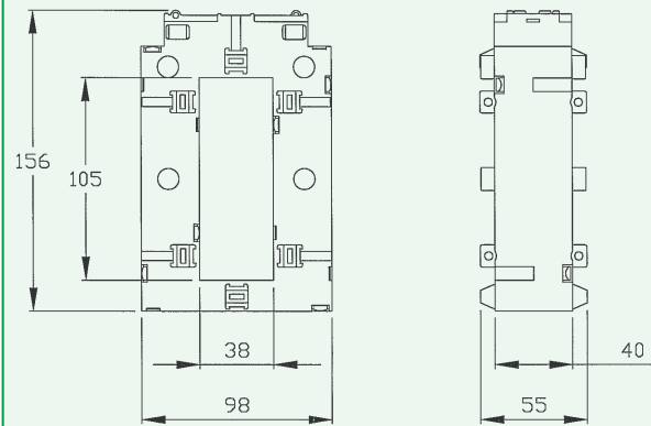
FOX105.38 DIMENSIONS
