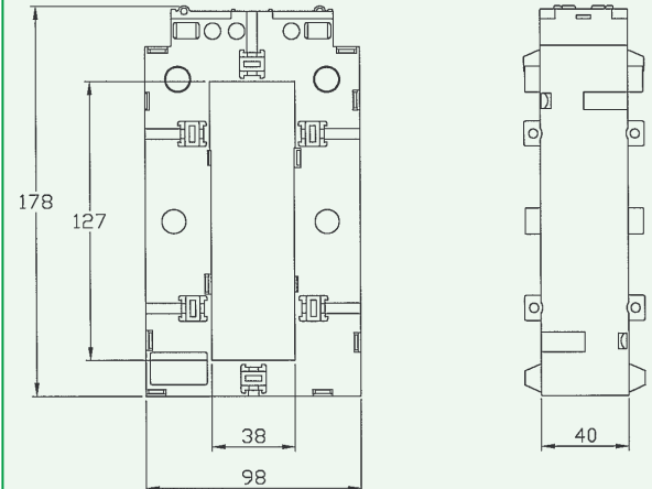
FOX127.38 DIMENSIONS
