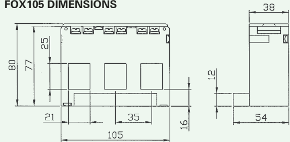
FOX105 DIMENSIONS
