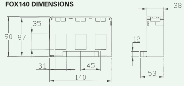
FOX140 DIMENSIONS
