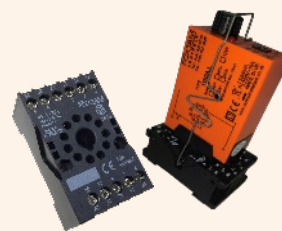
SCREW TERMINAL SOCKET PF-083BE, PF113BE
