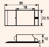
SCREW TERMINAL SOCKET PF-083BE, PF113BE
